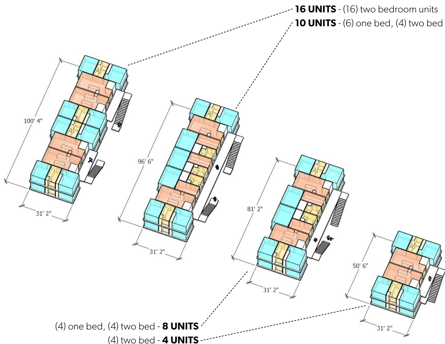
Figure 30: Unit Test Fitting
